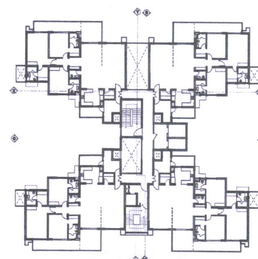
1 TYPICAL FLOOR KEY PLAN T-1 Scale: 1:500
